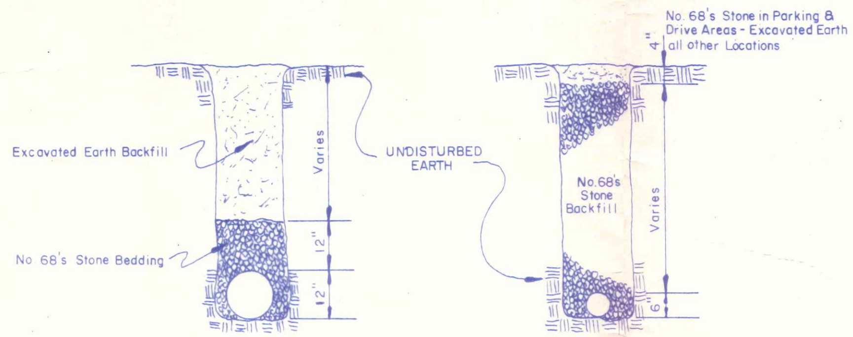
TYPICAL TRENCH 6" LATERAL TILE
