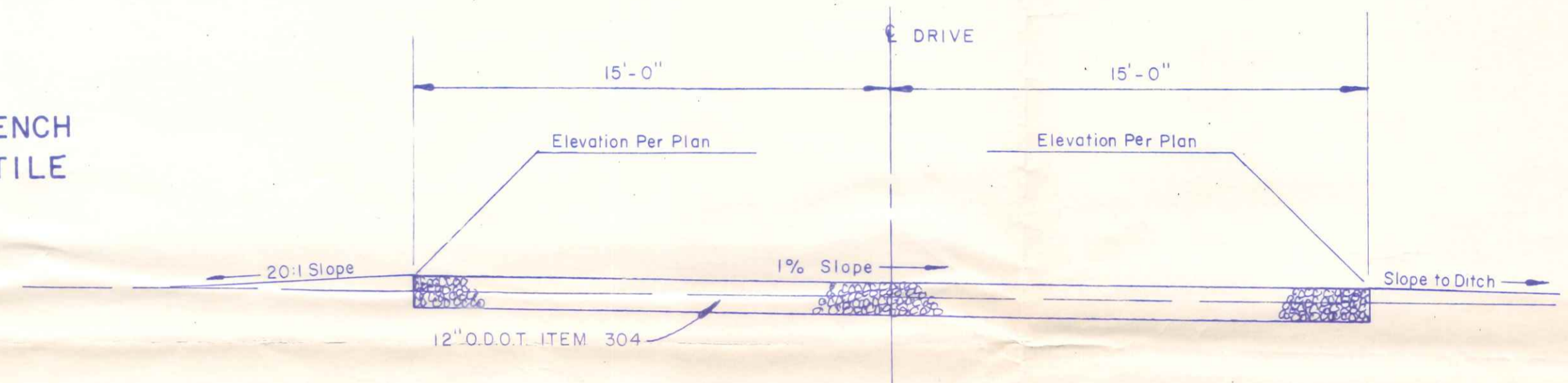
TYPICAL DRIVE SECTION
